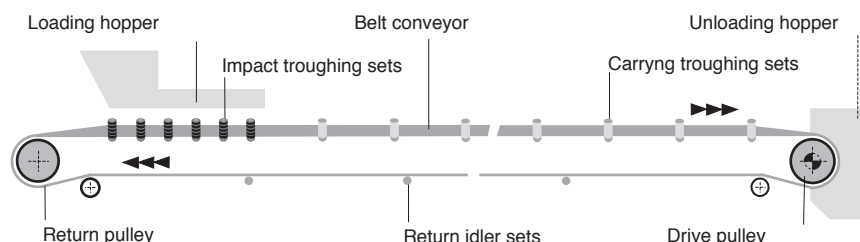
Fig.1 - Basic drawing of a belt conveyor
